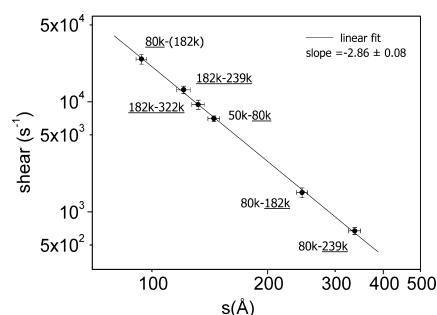
Figure 11. A log–log plot of critical shear rate, \dot{\gamma}_c , for chain detachment of bimodal brush systems versus interchain spacing, s , of polymeric chains that desorbed. The values of s and \dot{\gamma}_c are presented in Table 2. Each experimental point is labeled with the molecular weight pair of the bimodal copolymer system that exposed to shear flow. In each case, the component of the bimodal system that detached at the critical shear rate is underlined. The linear fit of experimental points yields a slope of -2.86 \pm 0.08 , indicating that the power law \dot{\gamma}_c \sim s^{-3} that was found previously for unimodal block copolymers 35 is also valid for bimodal systems.
