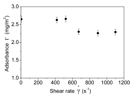
Figure 6. Change of adsorbance with shear rate for the 80K–239K PS–PEO bimodal brush system. Each point is calculated from the area under the volume fraction profile determined at each shear rate. Desorption of 239K PS–PEO component occurs at 672 s -1 .
