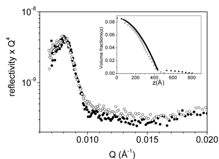
Figure 5. Reflectivity profile of bimodal 80K–239K PS–PEO diblock copolymer brush. Filled circles represent the measured static (zero shear) reflectivity profile while open circles indicate the profile after desorption of the 239K PS–PEO component of the brush at 672 s -1 . Inset: volume fraction profiles for above-described reflectivity profiles. Filled circles represent the volume fraction profile obtained from the best fit to the static (zero shear) reflectivity profile using the two-parabola model while open circles show the profile after the desorption of 239K PS–PEO at 672 s -1 .
