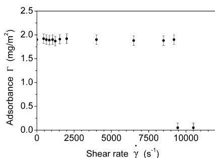
Figure 9. Adsorbance values of the 182K–322K PS–PEO bimodal brush system as a function of shear rate. No detachment occurs at low shear rate (below 1000 s −1 ), which would be characteristic of desorption of the longer chains (322K). On the contrary, both molecular weights desorbed together at a shear rate of 9540 s −1 .
